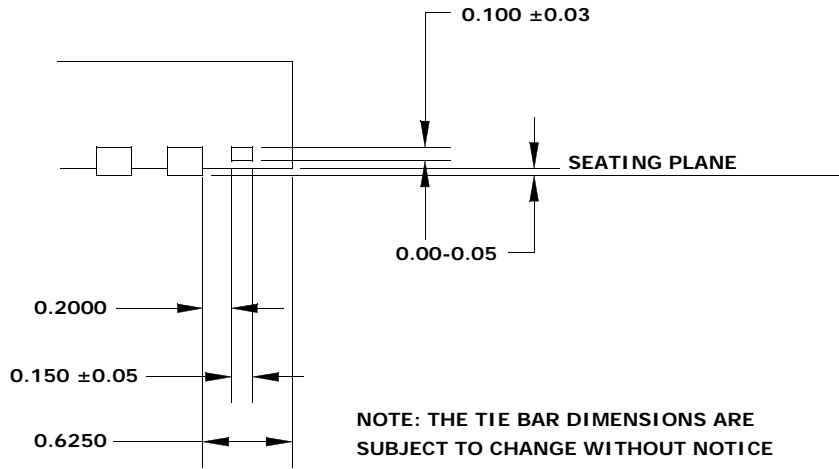
FIGURE 12. TIE BAR LOCATION FOR 4X5 QFN
