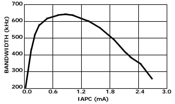
FIGURE 10. I OUT /I APC BANDWIDTH vs I APC
